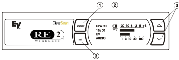
Figure 1 - RE-2 Front Panel
